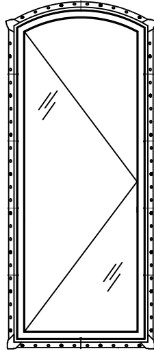
EXTERIOR ELEVATION
